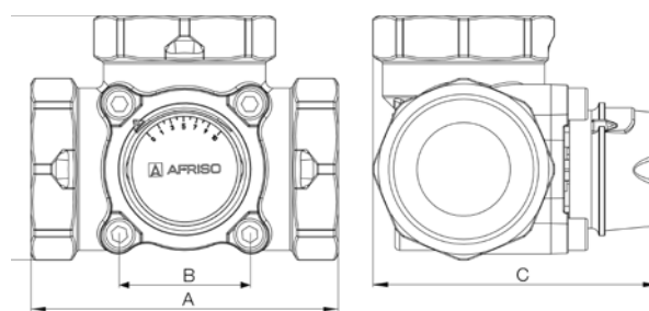
3-way mixing valve DN 40, 50
